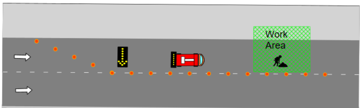
Figure 9: Shadow vehicle scenario 1 – Works in traffic lane on road with two lanes in one direction. Example illustrates where shadow vehicle has been positioned closer to work area and additional arrow board used at the beginning of the lane closure.
