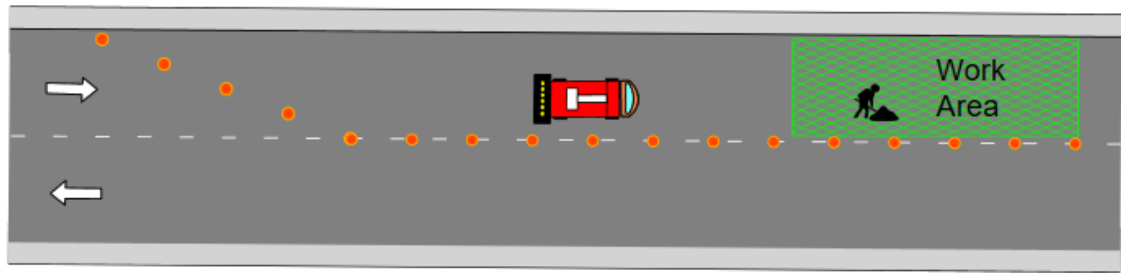
Figure 10: Shadow vehicle scenario 1 – Works in traffic lane of 2 lane 2-way road. Example illustrates the shadow vehicle positioned to protect workers from the direction of traffic flow in the closed lane.
