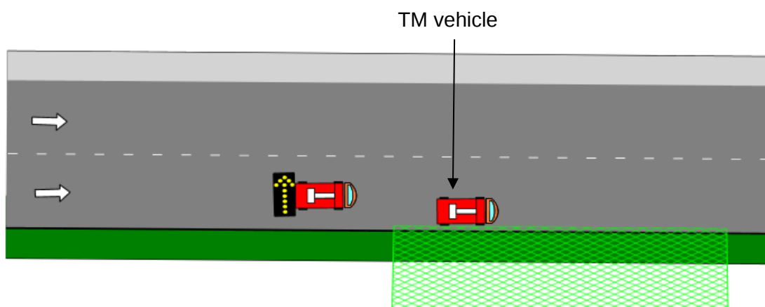
Figure 12: Shadow vehicle scenario 1 – Setting up traffic management from traffic lane. Note example shows scenario where traffic management is required on a kerbed median island.
