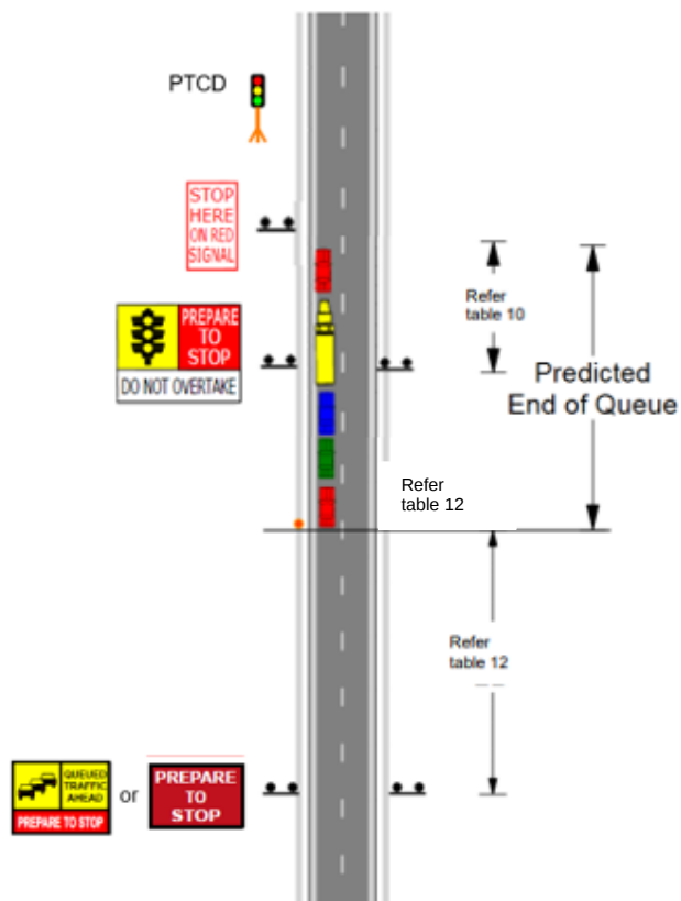
Figure 4: Avoiding end of queue collision
