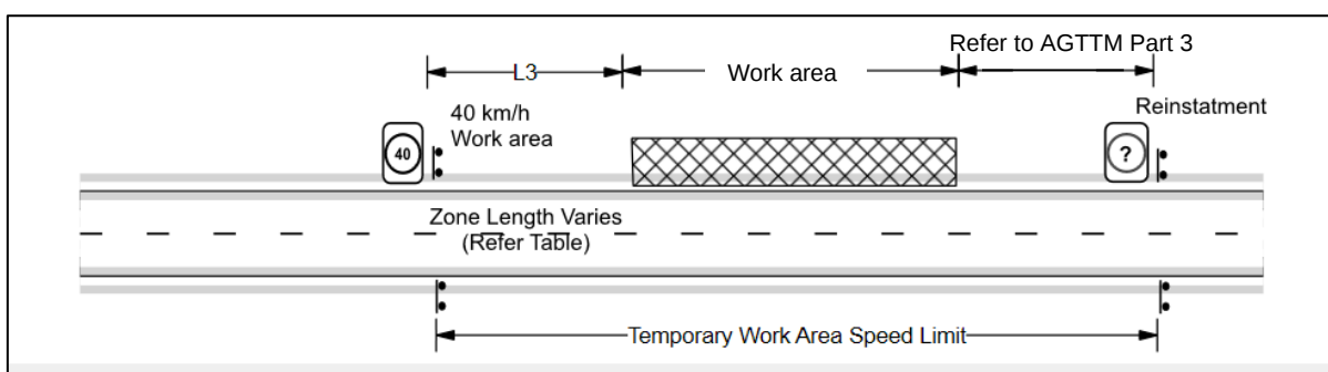
(b) No buffer zone required with 40 km/h work area speed limit (where posted speed limit less than 80 km/h).
