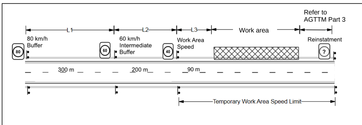
(a) Buffer zones – 110 km/h to 40 km/h
