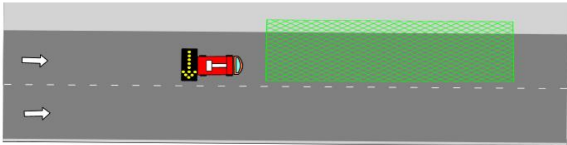
Figure 11: Shadow vehicle scenario 1 – Setting up traffic management within traffic lane on road with two lanes in one direction.
